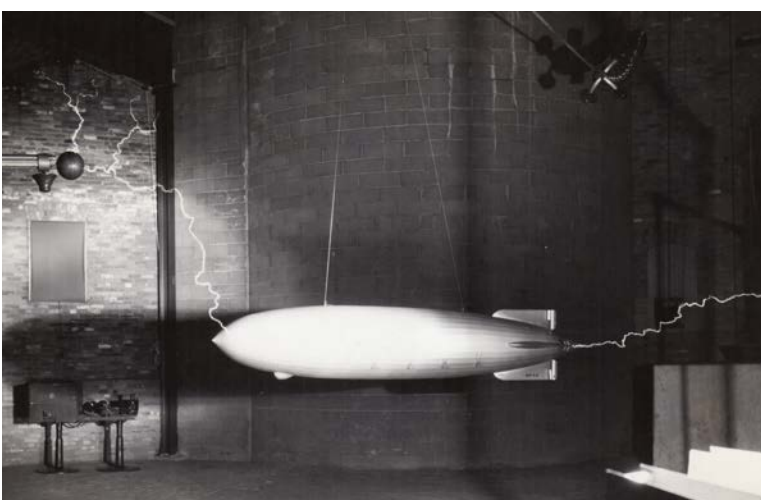
Airship lightning test in A.O. Austin's laboratory. Photo from the Akron Beacon Journal Collection.
