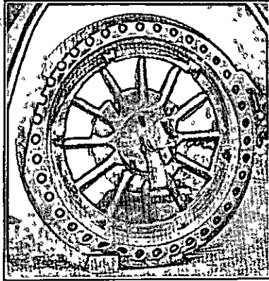
Note oblong shape of air holes at bottom of Lambert 'Trublpruf' Tire
