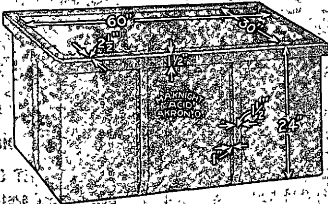
FIGURE 232—LARGE SIZE ONE PIECE TANK
