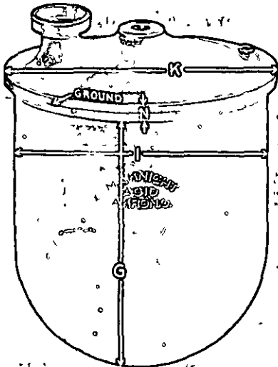
Figure 181 Acid Proof Nitrating Kettle and Cover
