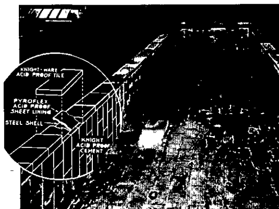
Pyroflex Constructed Pickling Tank in strip steel mill.
