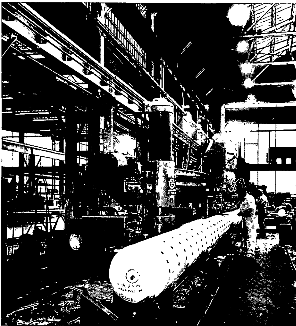
EMPLOYEES AT B & W'S BARBERTON WORKS USE MODERN EQUIPMENT TO DRILL HOLES IN HEADER COMPONENTS SUCH AS THESE ARE USED IN STEAM GENERATING EQUIPMENT
